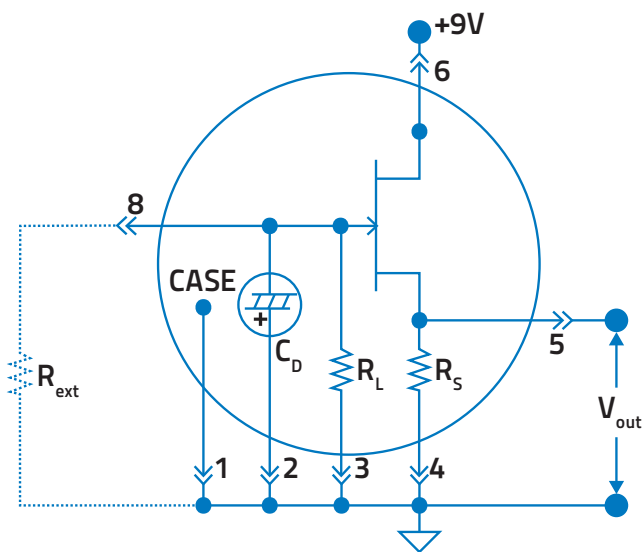
Figure 4: QS-VL circuitry
