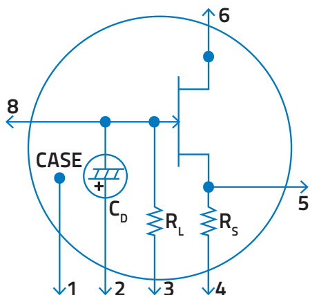
Figure 3: QS-VL Pin-Out
