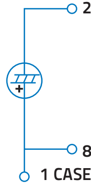
Figure 6: QS-H Pin-Out
