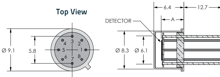
Figure 7: QS detectors mechanical details (T05-Based)
