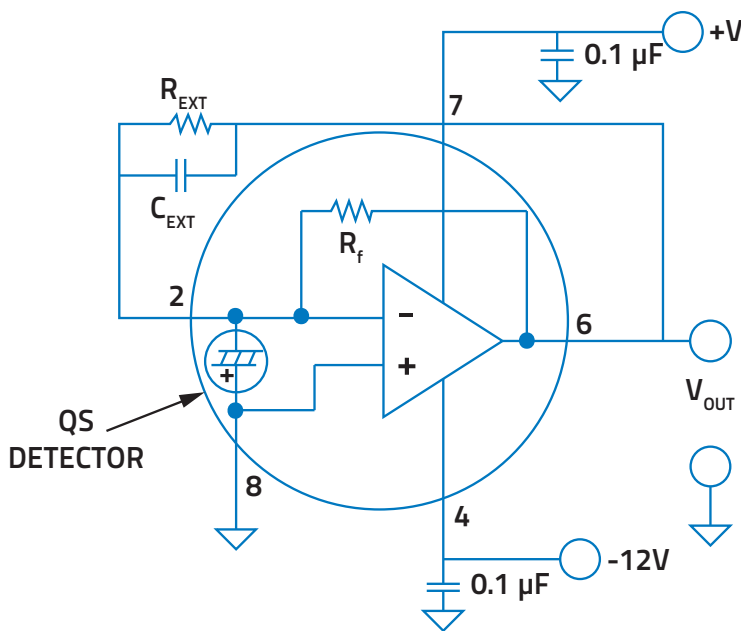
Figure 2: QS-IL, QS-IF and QS-THZ circuitry
