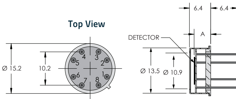
Figure 8: QS detectors mechanical details (T08-Based)
